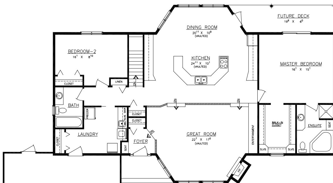
FLOOR PLAN
