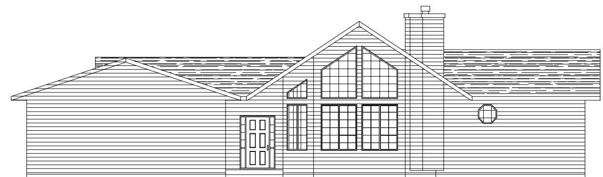
FRONT ELEVATION
